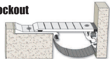
Model BIS-C Slab-to-Wall / Movement 2.5" to 12.5" Bolt-In Seismic Low Profile Design
