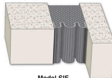
Model SIF Wall Corner / Movement .25" to 12.0"
