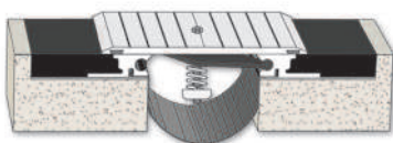
Model STS Top Mount/Slab-to-Slab Movement 1.0" to 18"
