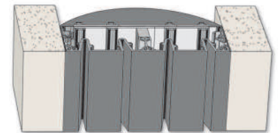
Model VSS Wall-to-Wall / Seismic Nominal Joint Openings 7" to 10" Movement 4" to 24"
