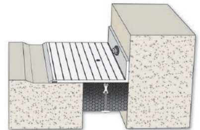
Model SHS-C Slab-to-Wall / Movement 2" to 27"
