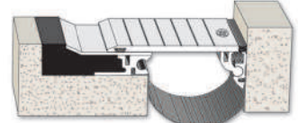
Model SSP-C Recessed/Slab-to-Wall Movement 1.75" to 15"
