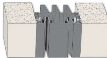
Model VSS Wall-to-Wall / Thermal Nominal Joint Openings 2" to 6" Movement 1.25" to 17"
