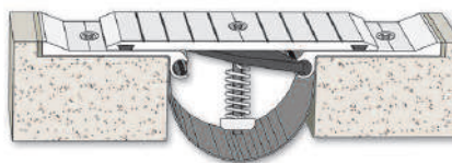
Model BIS Slab-to-Slab / Movement 2.5" to 15.0" Bolt-In Seismic Low Profile Design
